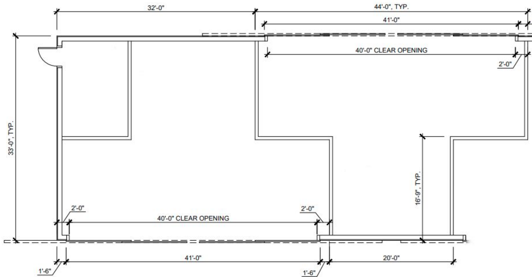
T Hangar Dimensions
