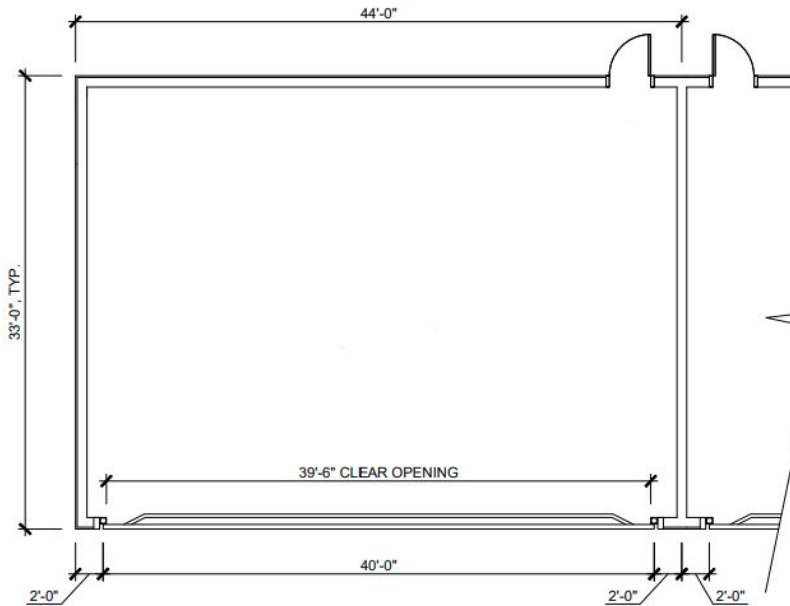
Box Hangar Dimensions
